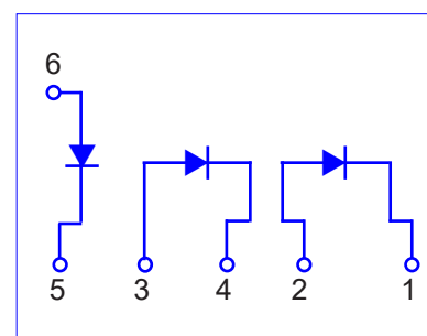
Schematic - CDA
