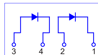
Schematic - CDA
